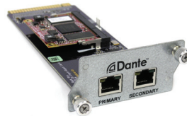
Dante Card Connects 16 channels of simultaneous audio input and output with Dante-enabled equipment
